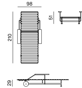
SUNLOUNGER + ARMRESTS dimensions 98 x 210 x 51 cm
