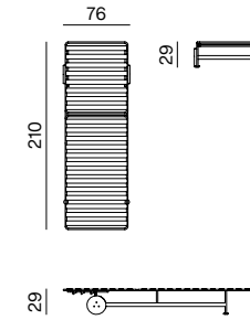
SUNLOUNGER dimensions 76 x 210 x 29 cm
