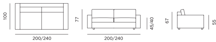
3SJED + MADRAC / 3SEATER + MATTRESS 2,5SJED + MADRAC / 2,5SEATER + MATTRESS
